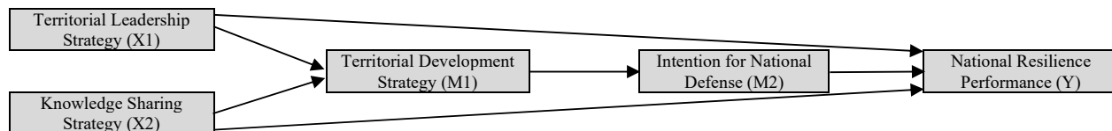
Fig. 1. Research framework
