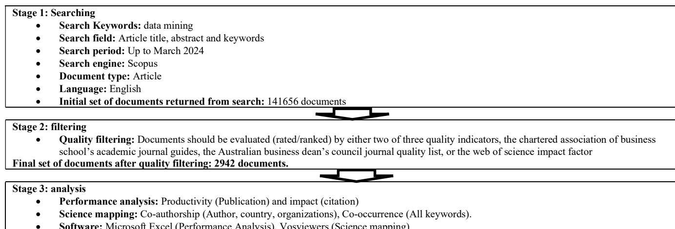
Fig. 1. Corpus curation
