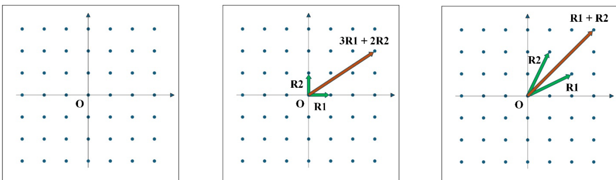
(a) A 2-dimensional lattice (b) An example of a short basis (c) An example of a long basis
