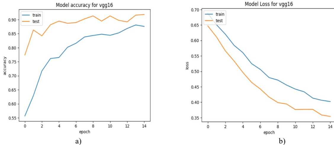
Fig. 19. Learning curves for (a) training and testing accuracy, and (b) training and testing loss of the VGG16 for Drones Forest Fire Detection Images 15 Epochs
