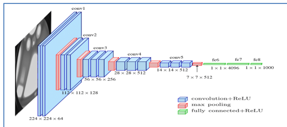
Fig. 5. VGG16 architecture (Nash et al., 2018)
