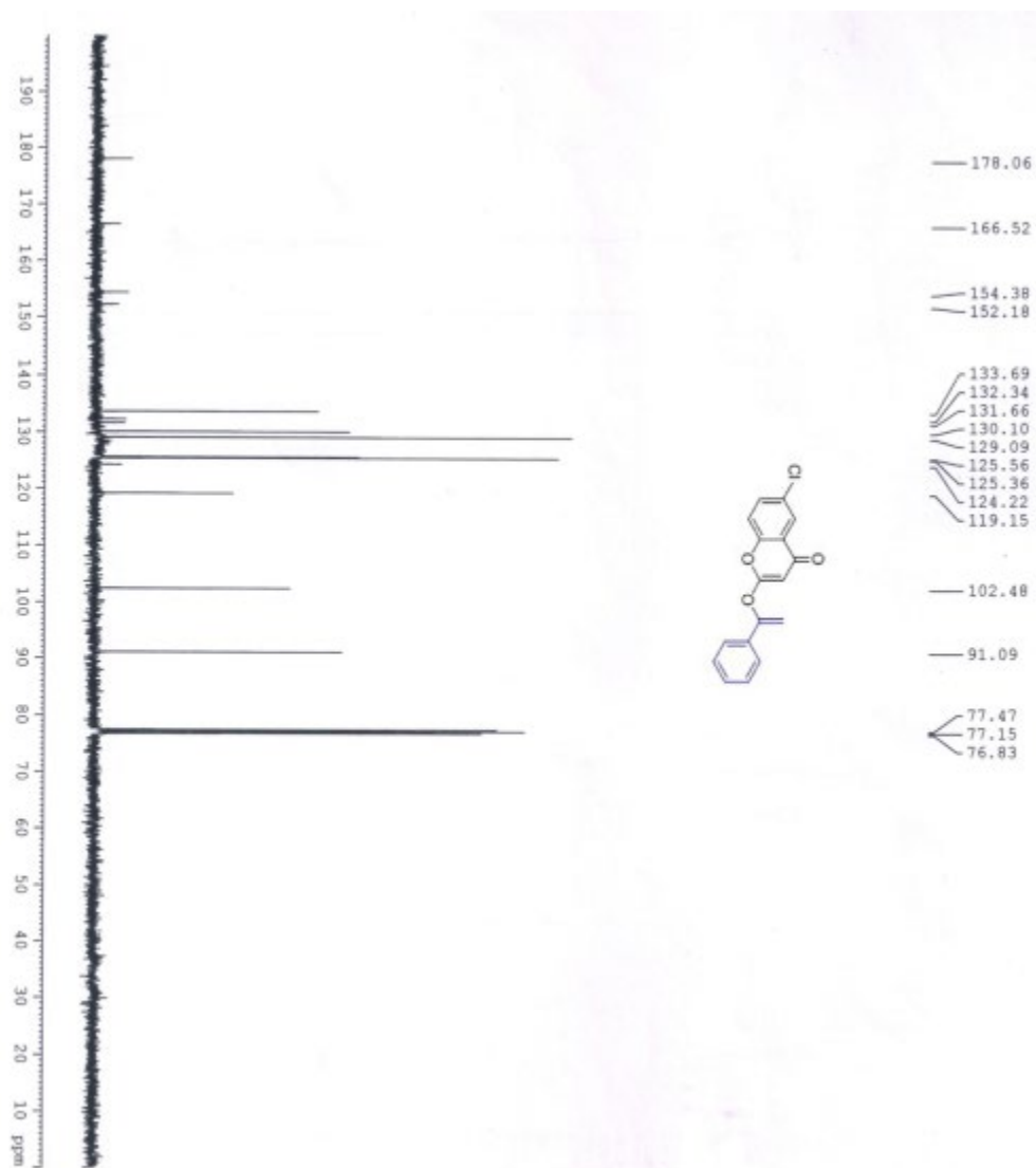
Figure 18. ^{13}\text{C} NMR spectrum of 3i
