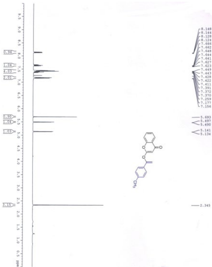
Figure 3. 1 H NMR spectrum of 3b
