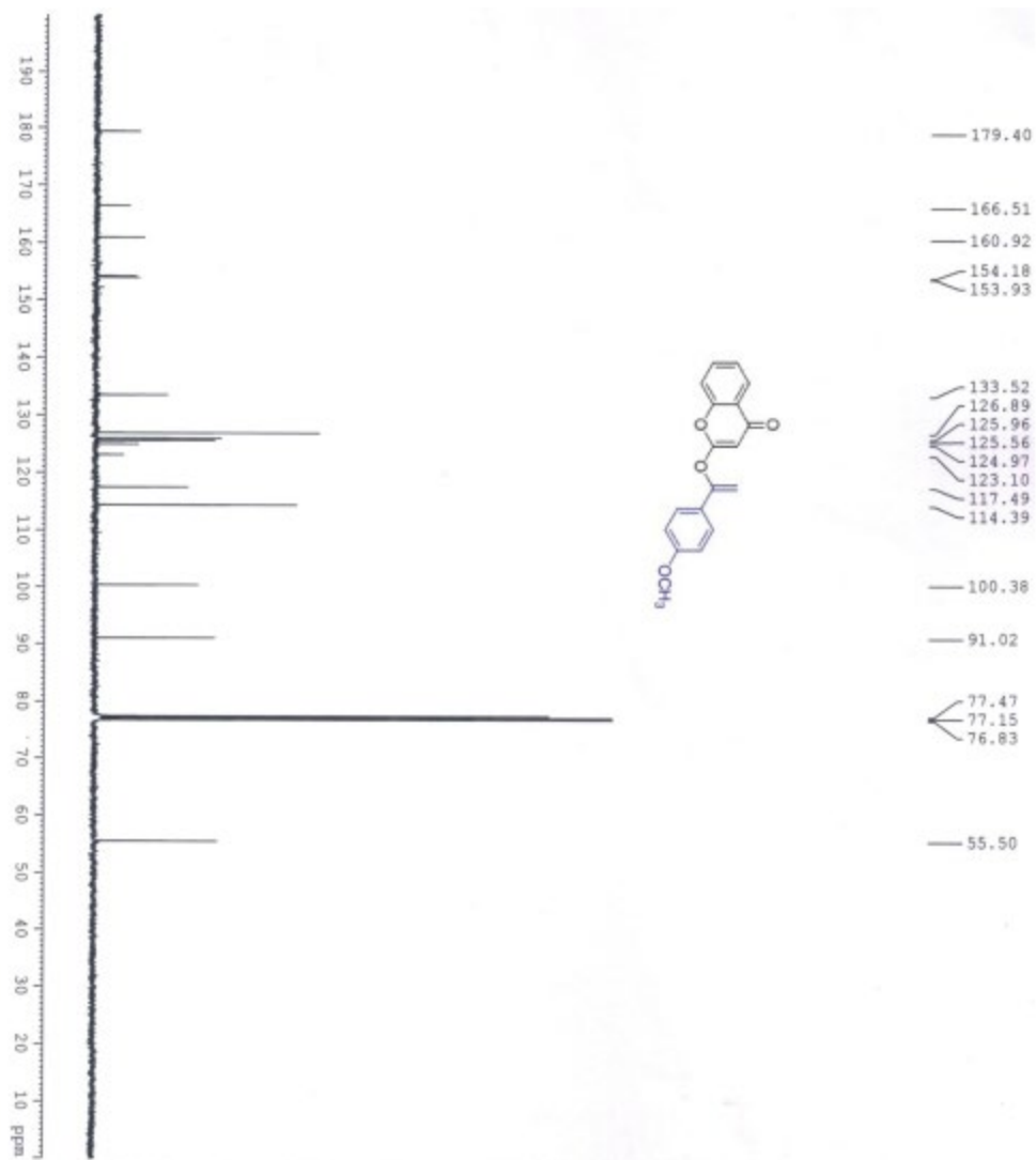
Figure 8. ^{13}\text{C} NMR spectrum of 3d
