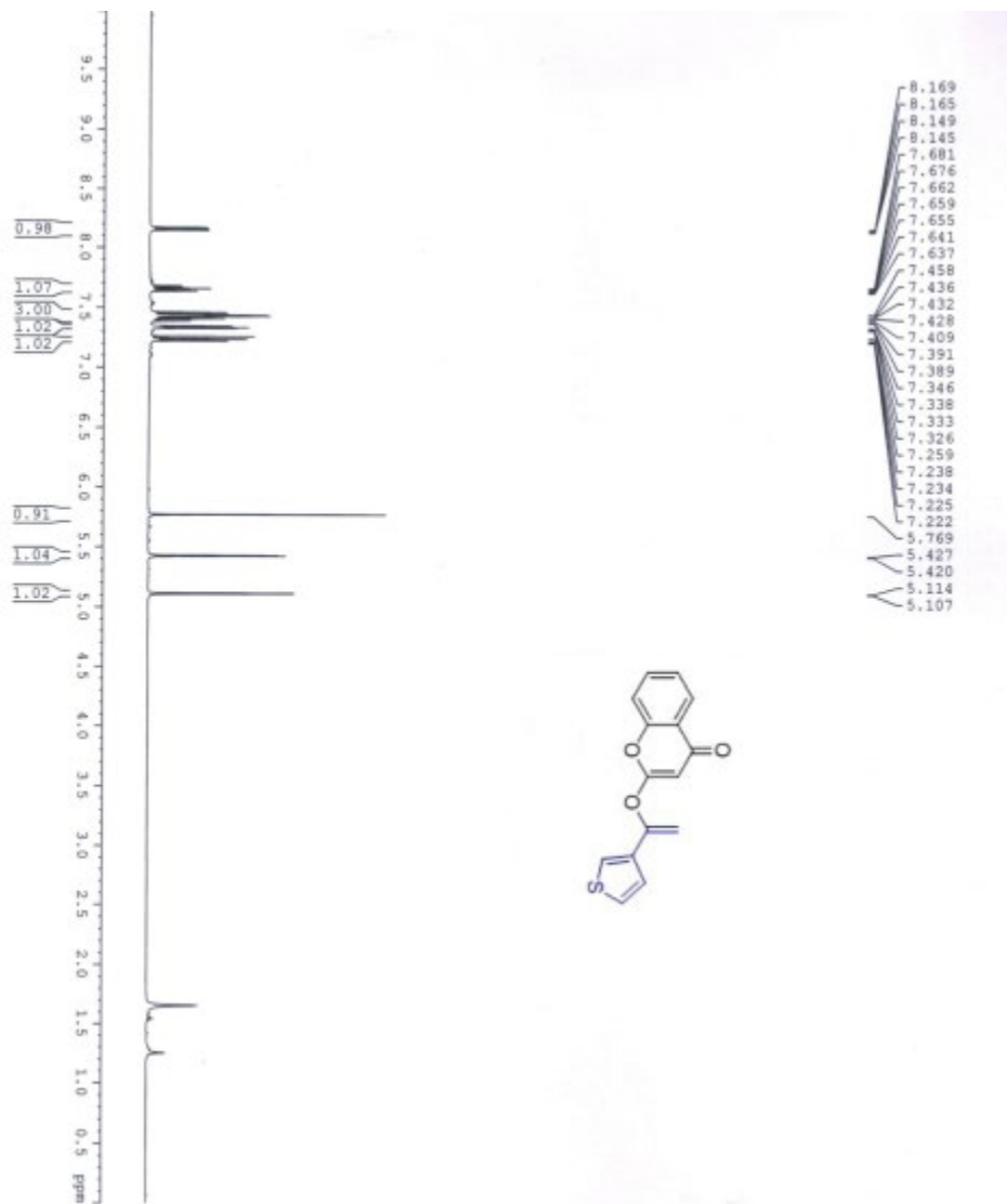
Figure 11. ^1\text{H} NMR spectrum of 3f
