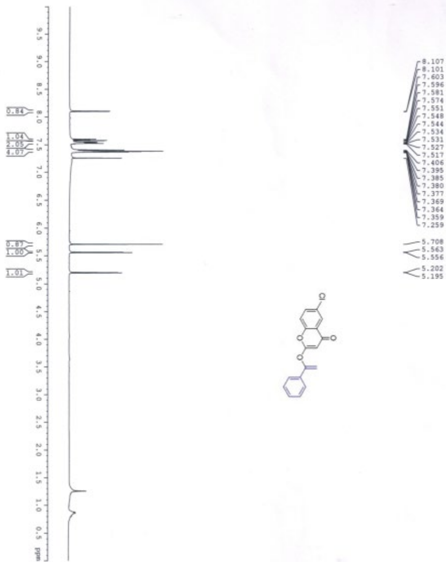
Figure 17. ^1\text{H} NMR spectrum of 3i
