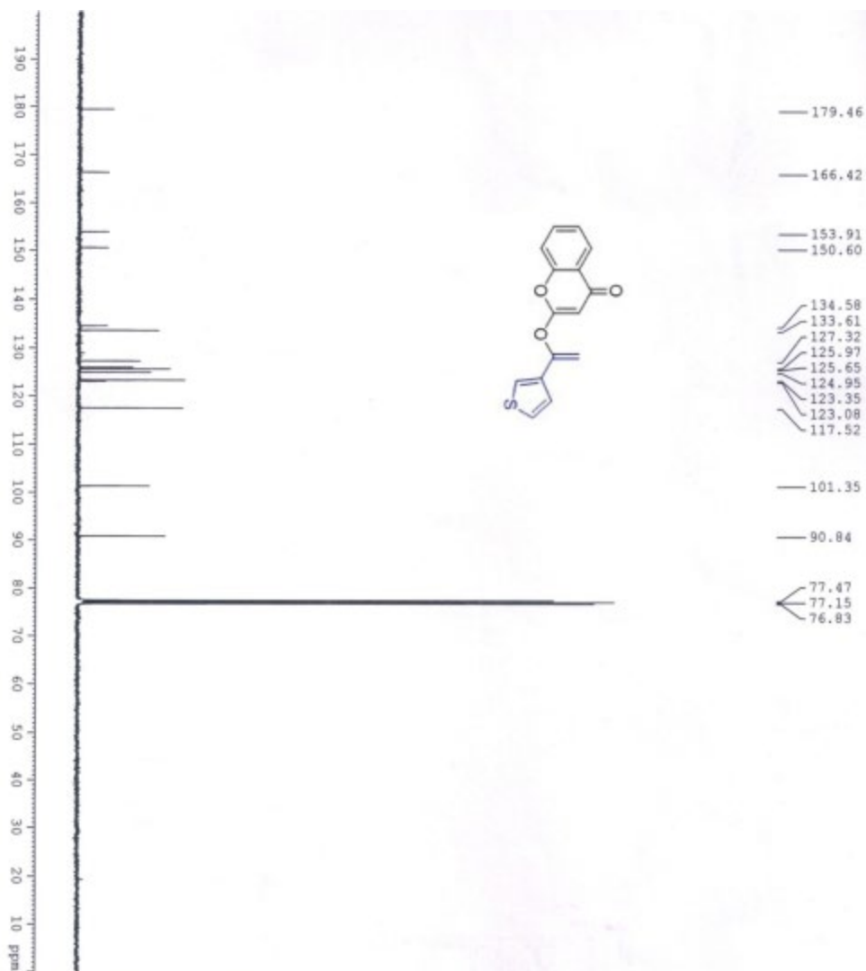
Figure 12. ^{13}\text{C} NMR spectrum of 3f
