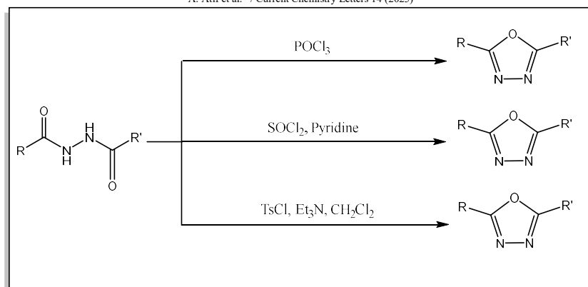
Scheme 3. Methods for the synthesis of 1,3,4-oxadiazole analogues from acylhydrazine derivatives.
