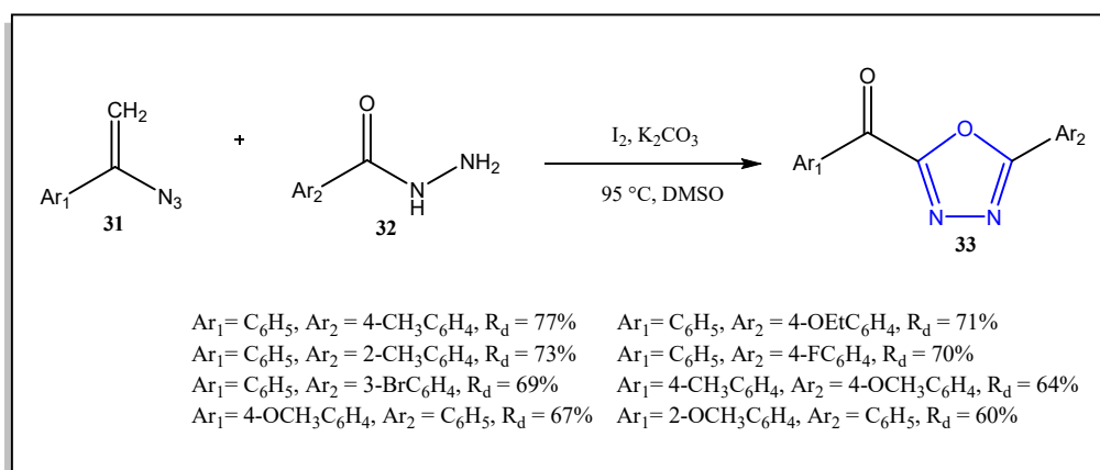
Scheme 9. Synthesis of 1,3,4- oxadiazole analogs by Swadhapriya Bhukta et al.
