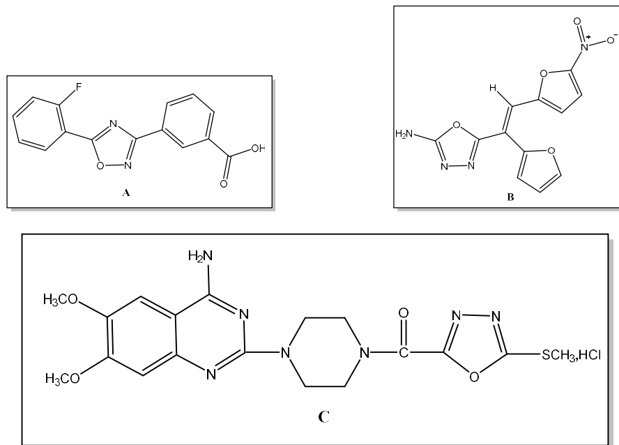
Fig. 2. (A) Ataluren, (B) Furamizole, (C) Doxazosine levulinate
