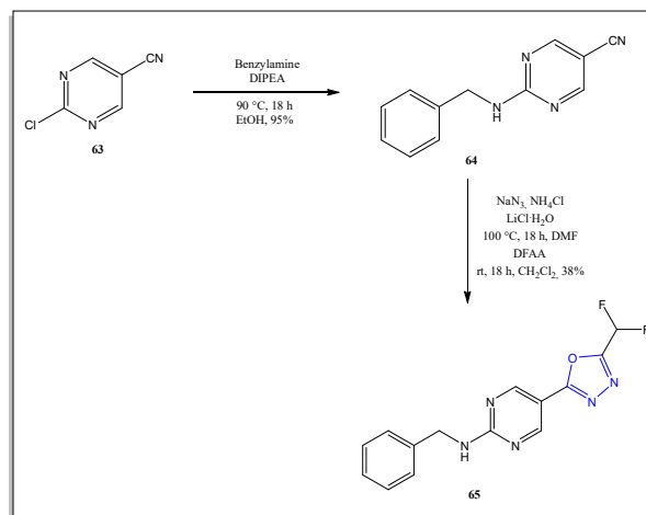
Scheme 18. Synthesis of 1,3,4- oxadiazole analogs by Beate König et al. ( procedure A )
