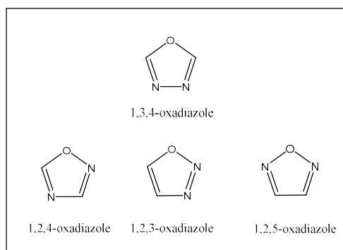
Fig. 1. General structure of 1,3,4-oxadiazole and isomers.
