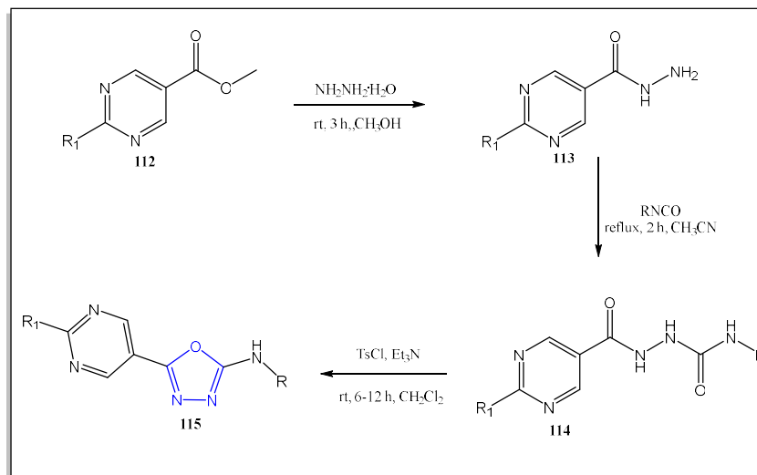
Scheme 29. Synthesis of 1,3,4-oxadiazole analogs by Vaclav Pfler et al.
