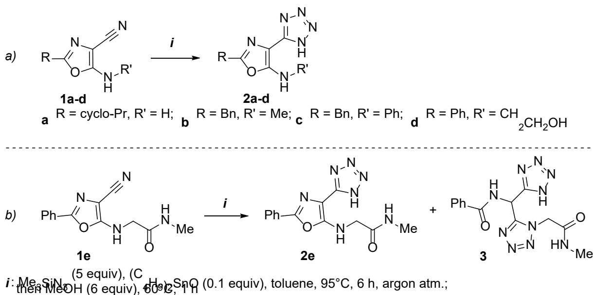
Schemes 3. The transformation of the substrates 1a-d nitrile group into tetrazole cycle.
