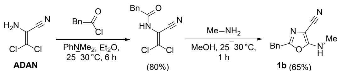
Schemes 2. The synthetic pathway for the compound 1b .
