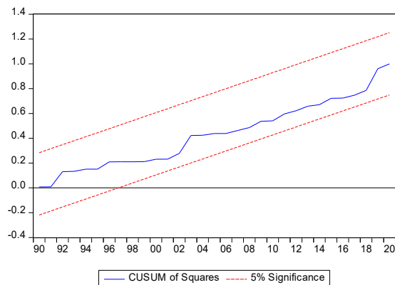
Fig. 2. CUSUMSQ Test
